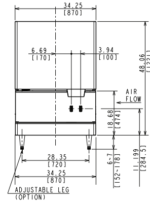
WATER-COOLED
