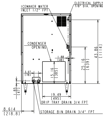
AIR-COOLED
